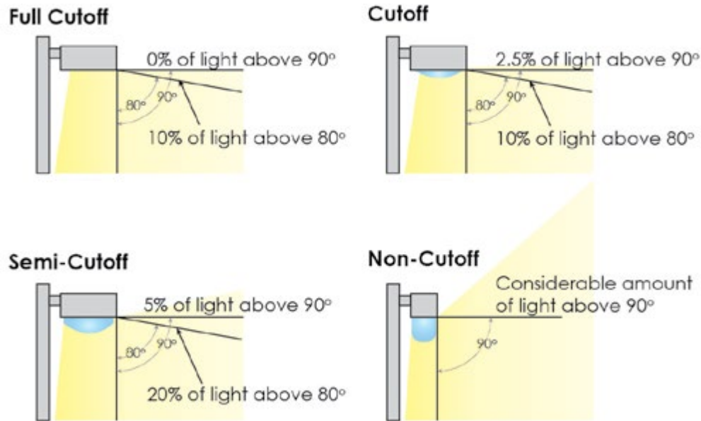
Figure 8 Lighting
