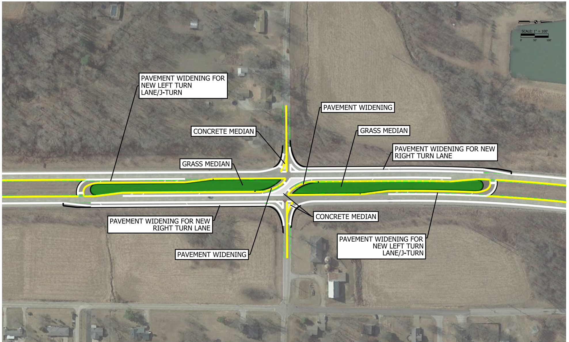
Figure 3-6 Typical J-Turn Alignment
