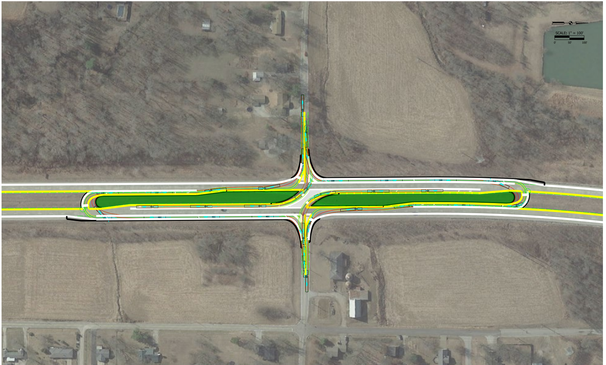
Figure 3-7 J-Turn n Truck Movements
